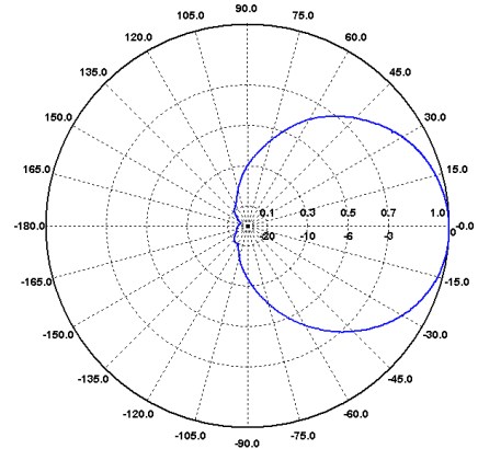
H-Ebene / H-Plane 500 MHz
