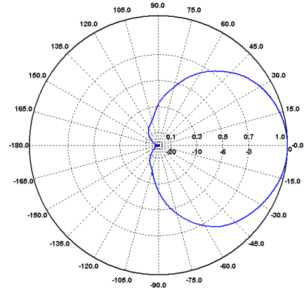
H-Ebene / H-Plane 600 MHz
