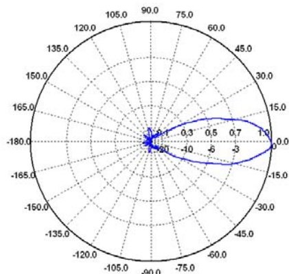
H-Ebene / H-Plane 1.8 GHz
