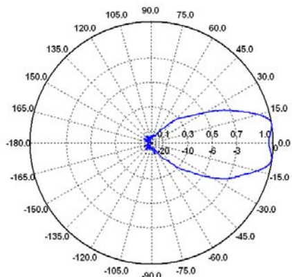
E-Ebene / E-Plane 1.8 GHz
