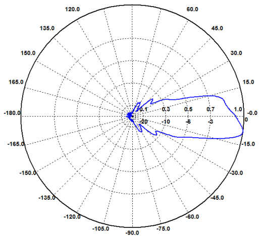
E-Ebene / E-Plane 8.0 GHz
