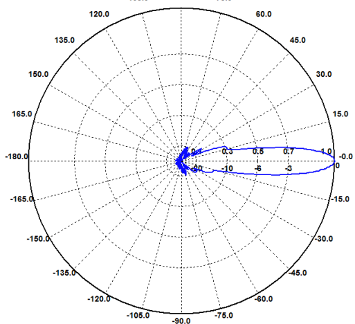
E-Ebene / E-Plane 9.0 GHz
