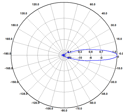
H-Ebene / H-Plane 8.0 GHz
