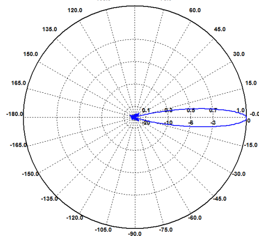
H-Ebene / H-Plane 9.0 GHz
