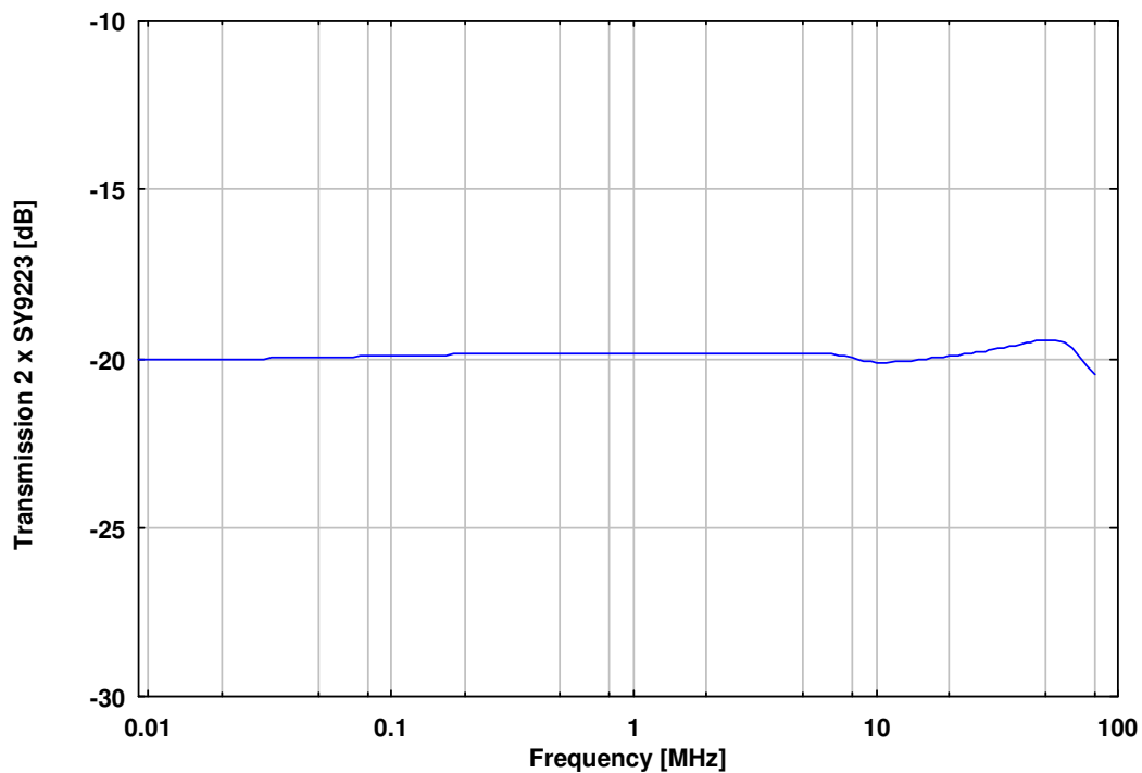
Abb. 1 Transmission zweier SY9223-100 an EuT verbunden Fig. 1: Transmission of two SY9223-100 connected at the EuT port
