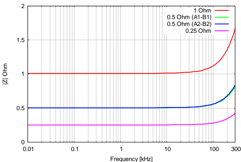
Typical impedance of Shunt 9571
