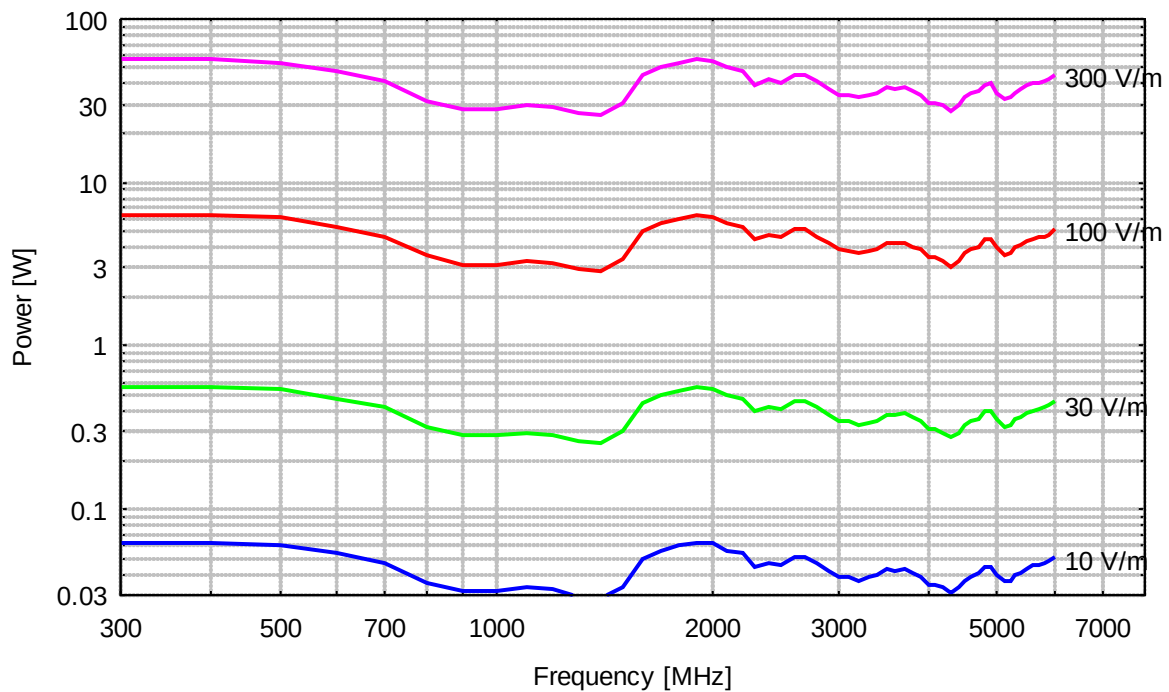
Power Requirement for constant Fieldstrength at 10 cm Distance
