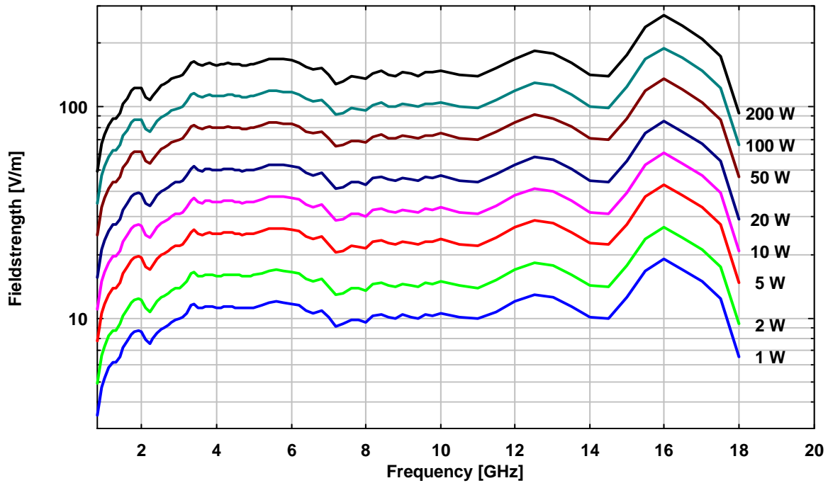
BBHA 9120 D Input Power, Dist. Aperture-EuT: 3 m
