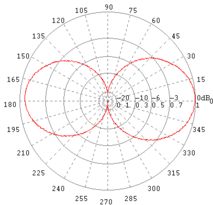
Richtdiagramm E-Ebene: Directional Pattern E-Plane:
